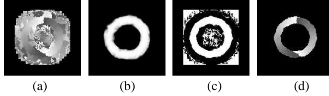
Figure 14: Translating Disk. (a) Raw orientation estimates from direct method. Black pixels indicate that no estimate was possible. Intensity varies from white to dark grey as orientation goes from \pi/2 to -\pi/2 . (b,c) Confidence measures from velocity constraint and orientation constraint. (d) orientation estimates masked by joint confidence measure.
